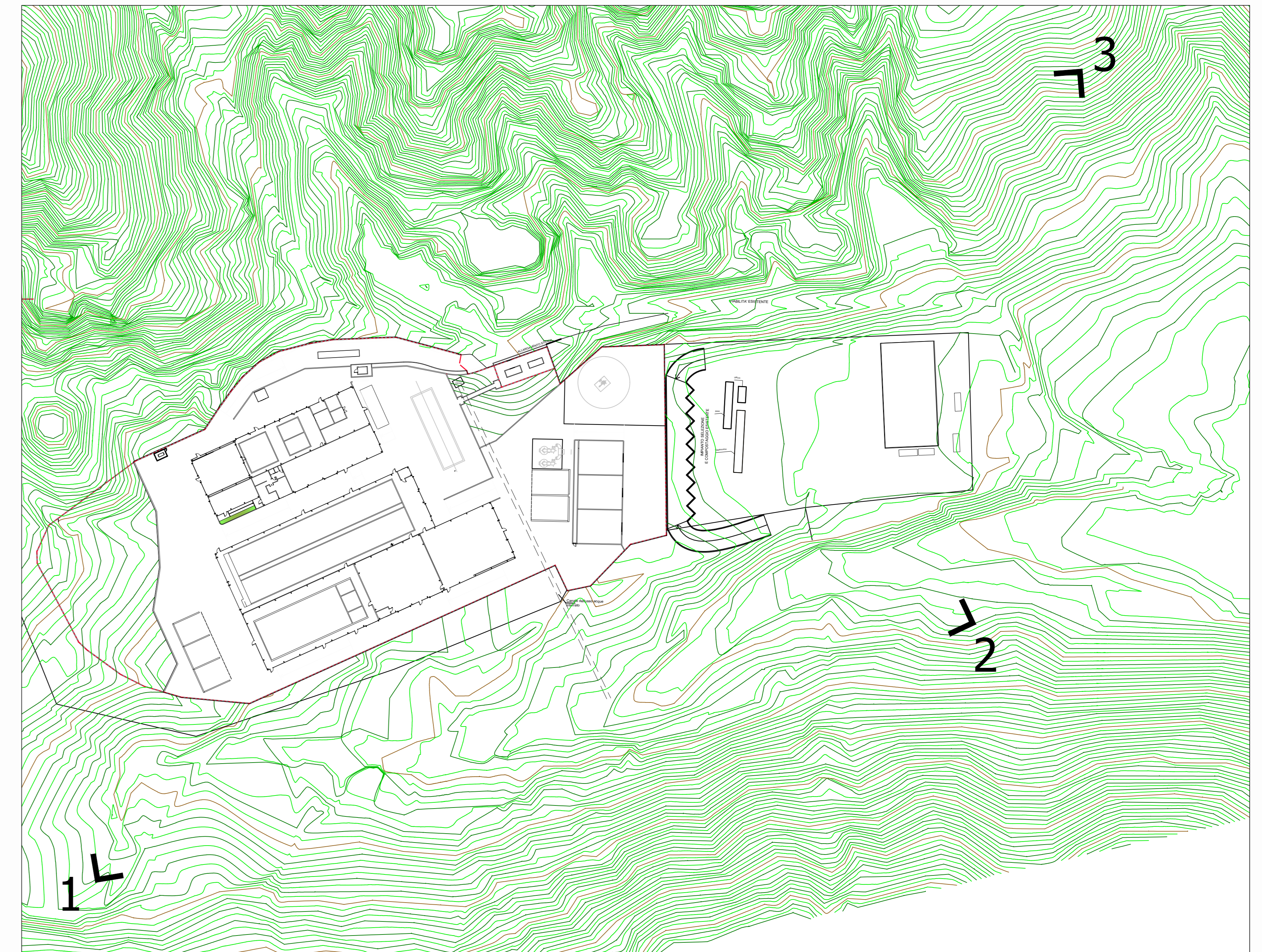
KEYPLAN
